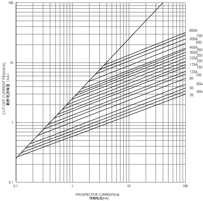
HBC截断电流曲线图 (仅供参考) HBC CUT-OFF CHARACTERISTICS CURVE (FOR REFERENCE)
