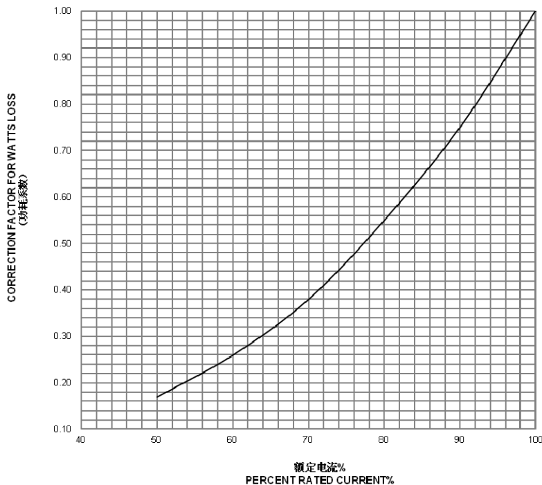
HBC电流功耗曲线图 HBC WATTS LOSS VS.% RATED CURRENT (FOR REFERENCE)
