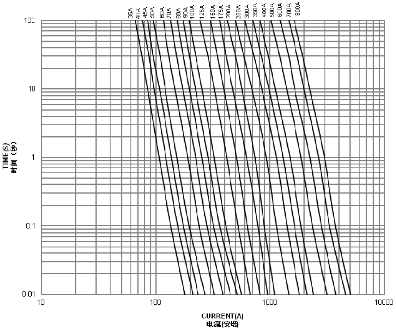
HBC平均 I-T 曲线图(仅供参考) HBC AVERAGE I-T CHARACTERISTICS CURVE (FOR REFERENCE)
